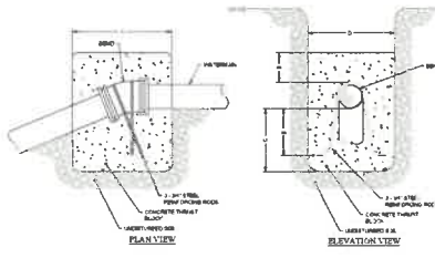
HORIZONTAL THRUST BLOCK NOT TO SCALE
