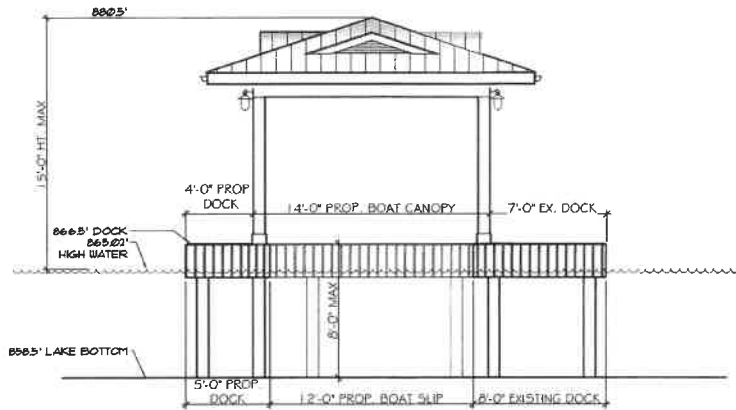
EAST ELEVATION
