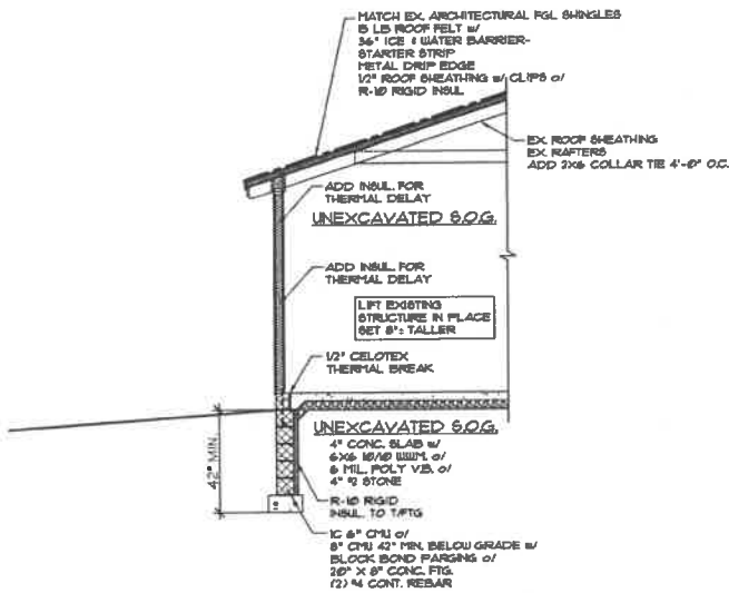
SECTION 'A' 1/4" = 1'-0"
