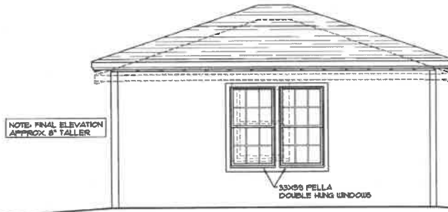
EAST ELEVATION 1/4" = 1'-0"
