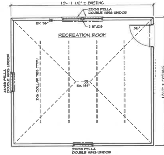
FIRST FLOOR PLAN 1/4" = 1'-0"
